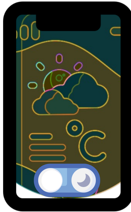
Dark Mode
